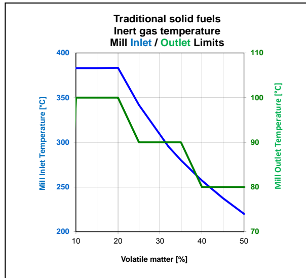
Figure 1: Grinding and drying operation temperatures
